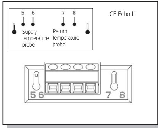
The color of the wires (polarity) is irrelevant
