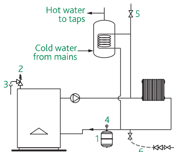
Fig. 3 - Typical System
